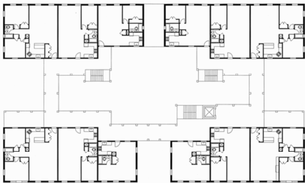
SECOND FLOOR PLANS
